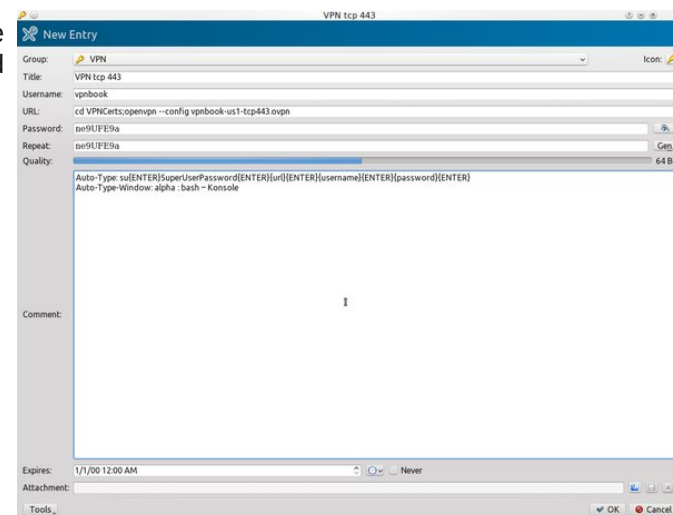
Sample of a filled entry in KeePassX.
